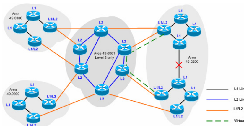
Figure 1. Typical ISIS Topology
